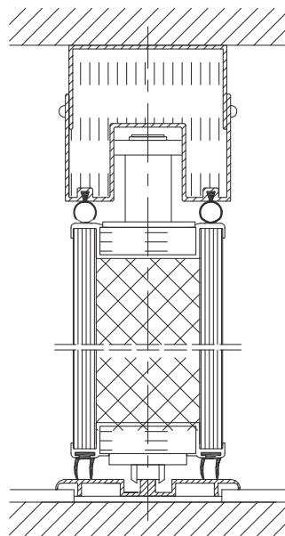
Floor track ceiling/floor connection
