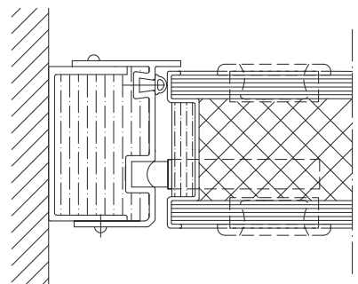
Wall connection - start profile
