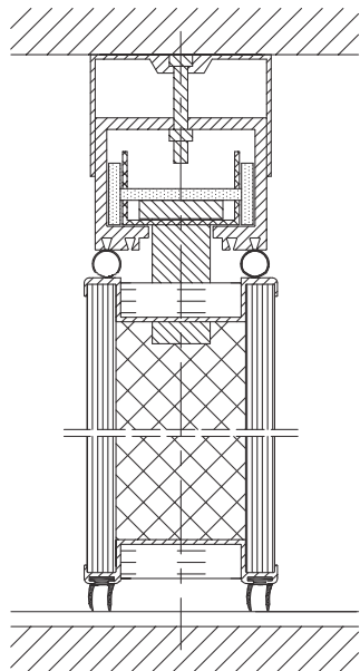
Top hung ceiling/floor connection
