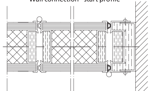
Wall connection - start profile
